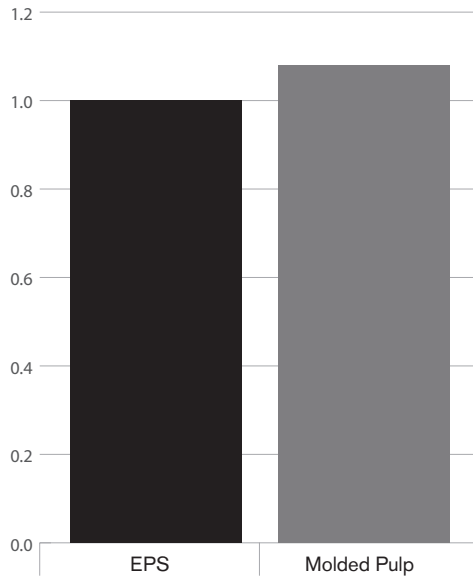
Figure 2: Climate Change comparison (EPS=1)
