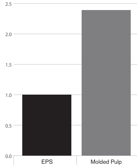
Figure 8: Eutrophication (Marine) comparison (EPS=1)
