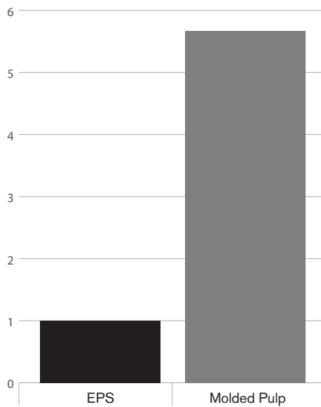
Figure 3: Water Use Volume comparison (EPS=1)
