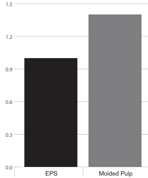
Figure 4: Cumulative Energy Demand comparison (EPS=1)
