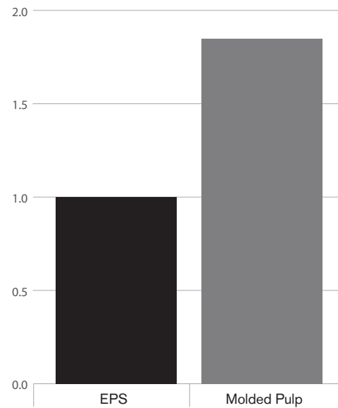
Figure 5: Ozone Depletion comparison (EPS=1)
