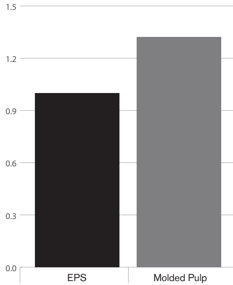
Figure 6: Acidification comparison (EPS=1)
