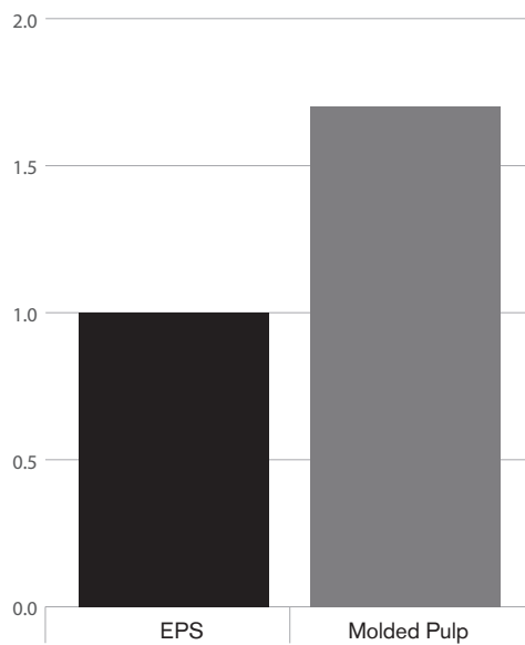
Figure 7: Photochemical Ozone Formation comparison (EPS=1)
